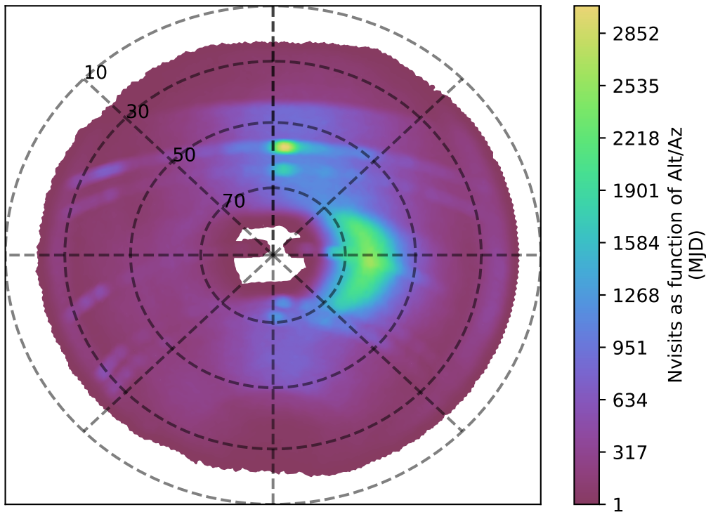
weather_cloudso2v3.4_10yrs i band: Nvisits as function of Alt/Az
