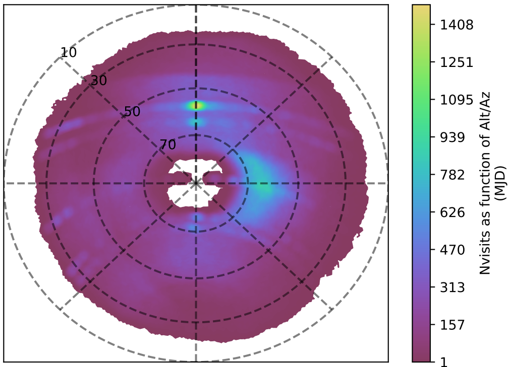
weather_cloudso2v3.4_10yrs g band: Nvisits as function of Alt/Az
