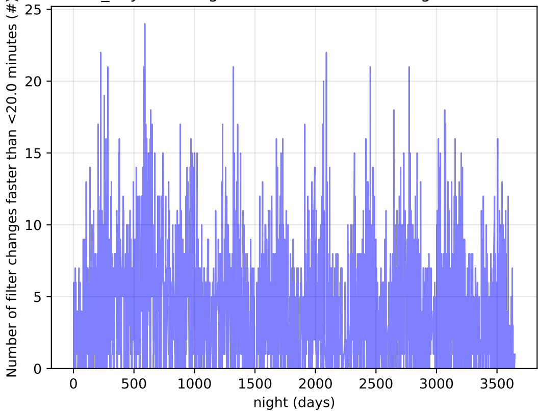
weather_cloudso2v3.4_10yrs Per Night: Number of filter changes faster than <20.0 minutes
