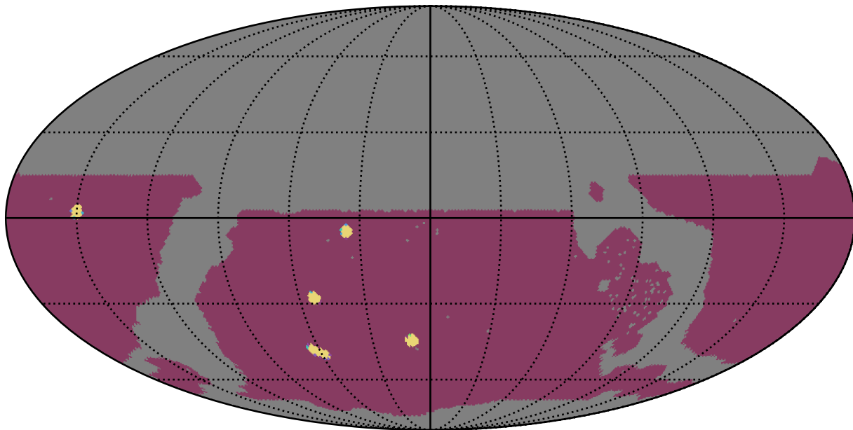
weather_cloudso2v3.4_10yrs WFD: NumberOfQuickRevisits
