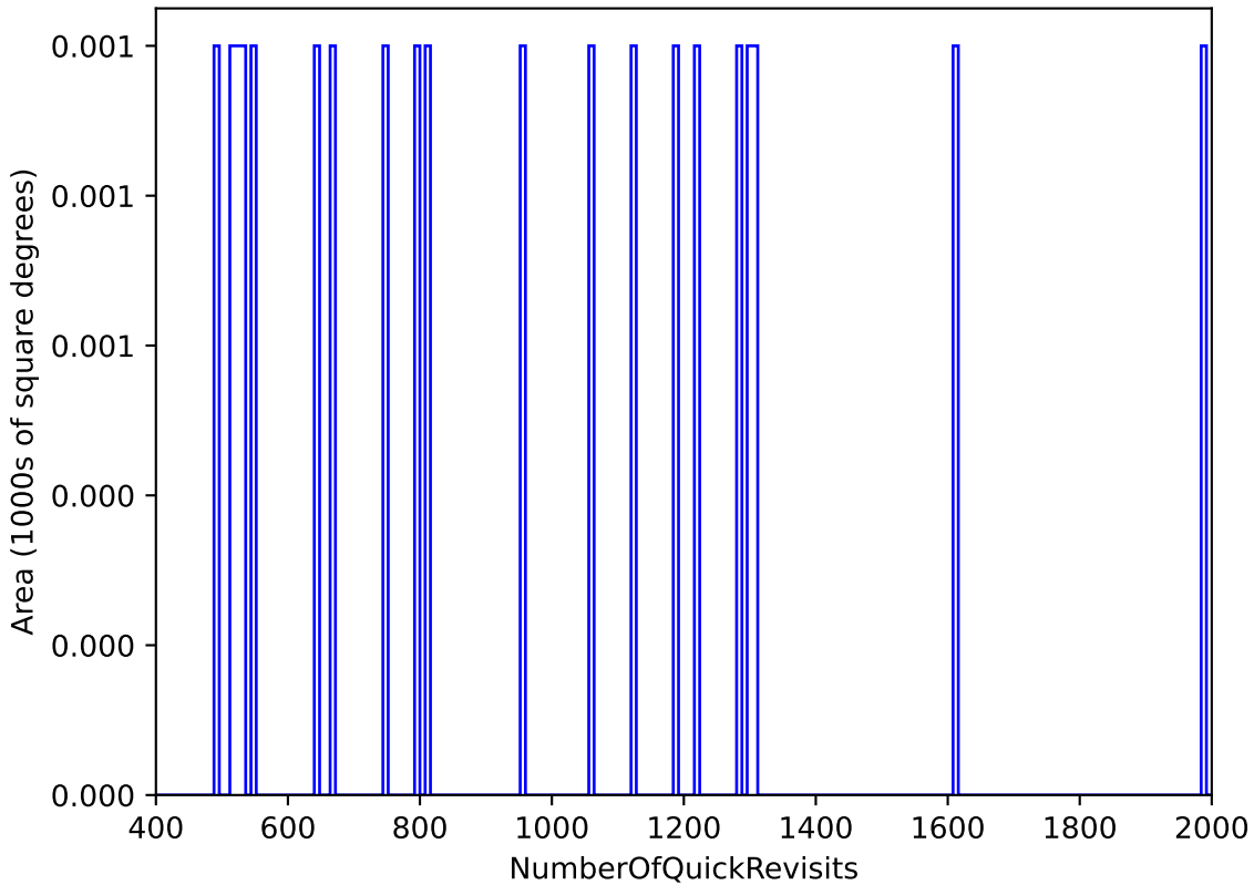
weather_cloudso2v3.4_10yrs WFD: NumberOfQuickRevisits
