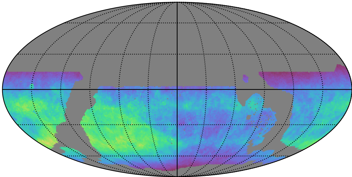
weather_cloudso2v3.4_10yrs WFD z band: Normalized Teff
