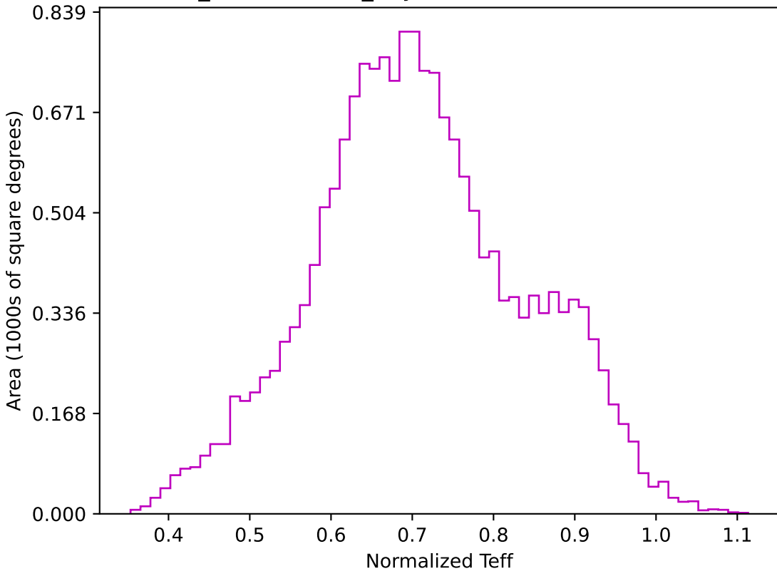
weather_cloudso2v3.4_10yrs WFD z band: Normalized Teff
