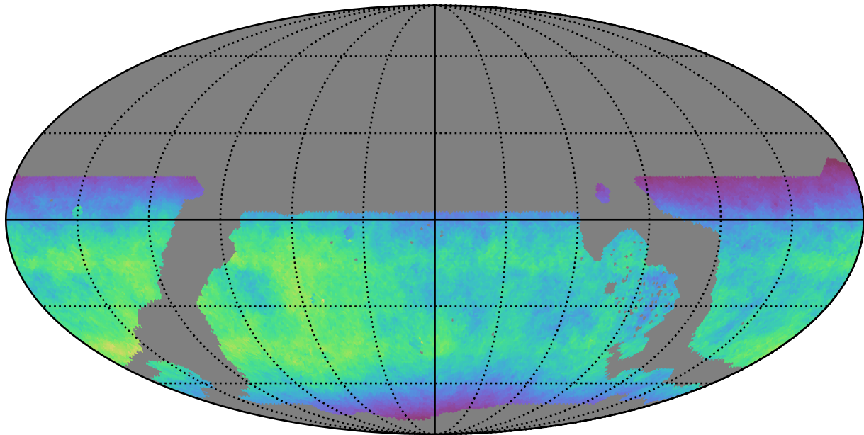
weather_cloudso2v3.4_10yrs WFD y band: Normalized Teff
