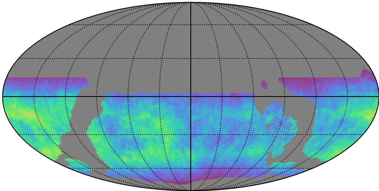
weather_cloudso2v3.4_10yrs WFD u band: Normalized Teff
