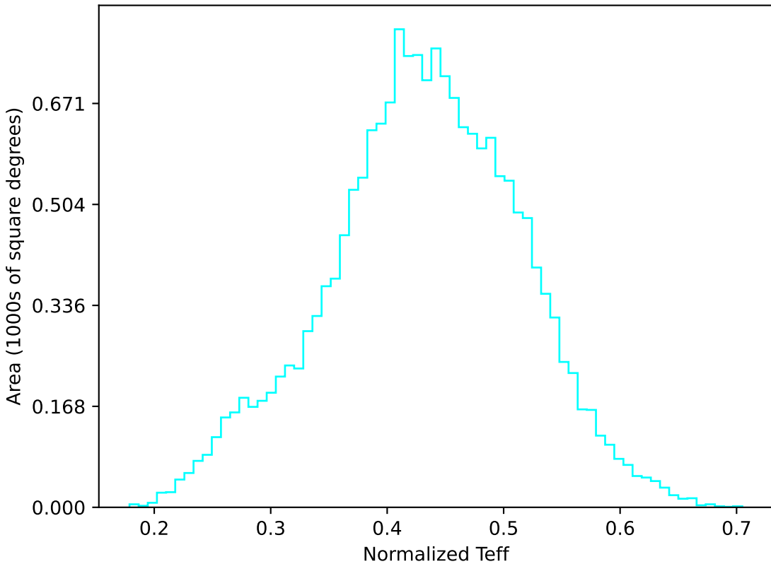
weather_cloudso2v3.4_10yrs WFD u band: Normalized Teff
