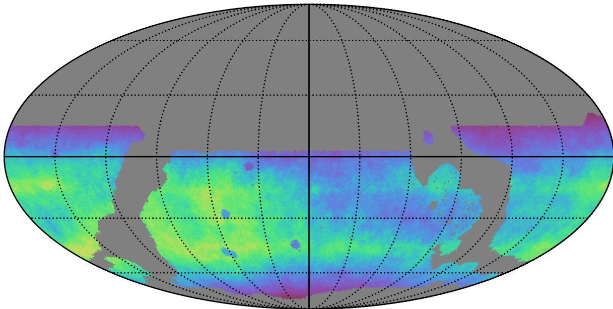
weather_cloudso2v3.4_10yrs WFD r band: Normalized Teff
