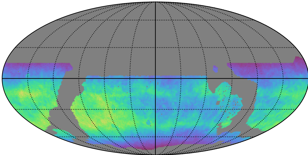
weather_cloudso2v3.4_10yrs WFD i band: Normalized Teff
