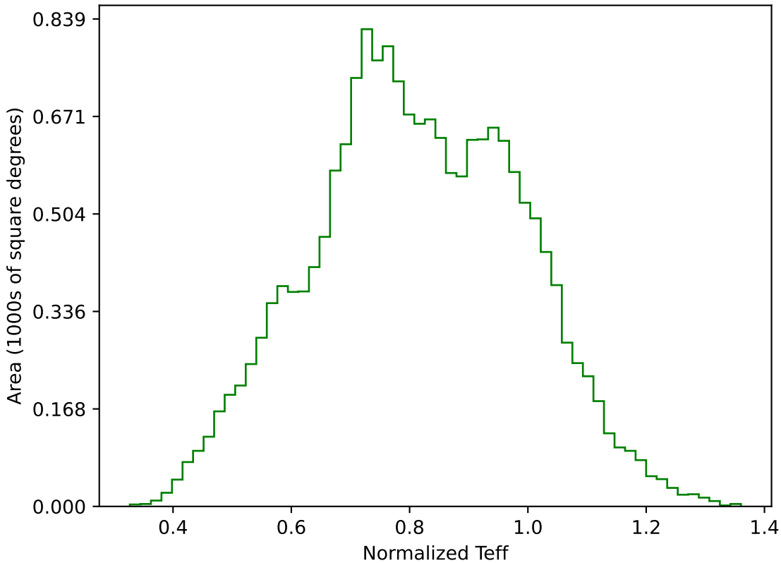
weather_cloudso2v3.4_10yrs WFD g band: Normalized Teff
