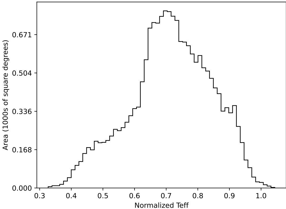
weather_cloudso2v3.4_10yrs WFD all bands: Normalized Teff
