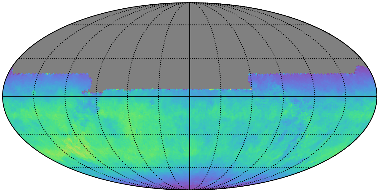
weather_cloudso2v3.4_10yrs All sky y band: Normalized Teff
