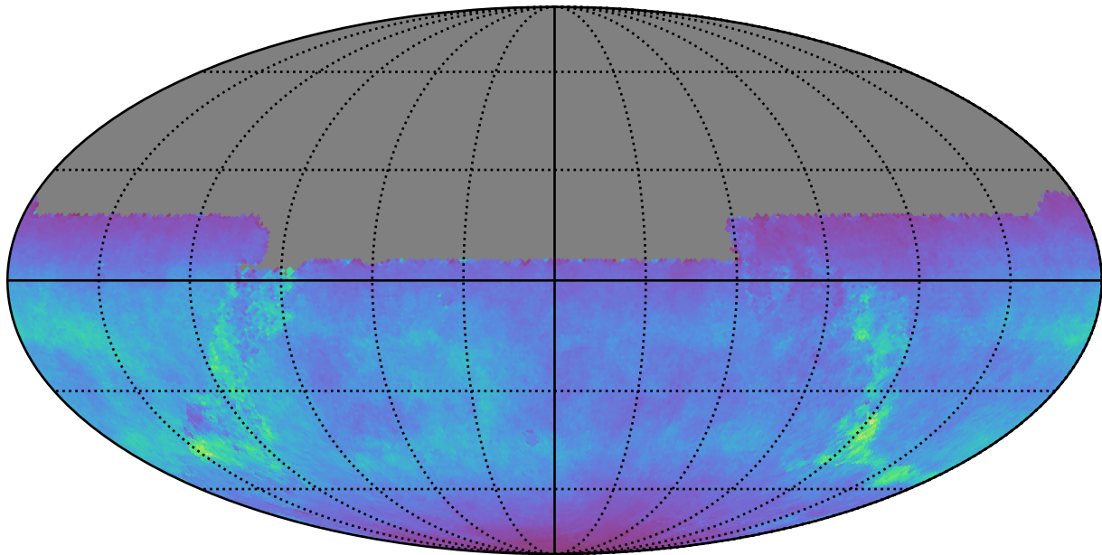
weather_cloudso2v3.4_10yrs All sky u band: Normalized Teff
