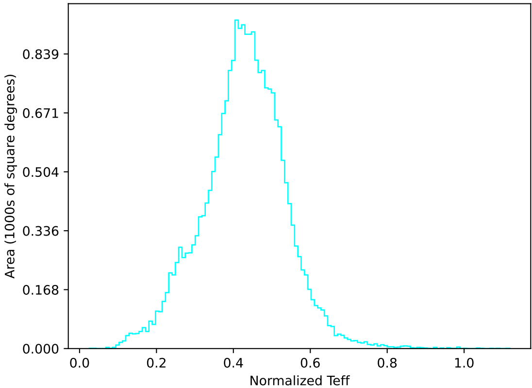
weather_cloudso2v3.4_10yrs All sky u band: Normalized Teff
