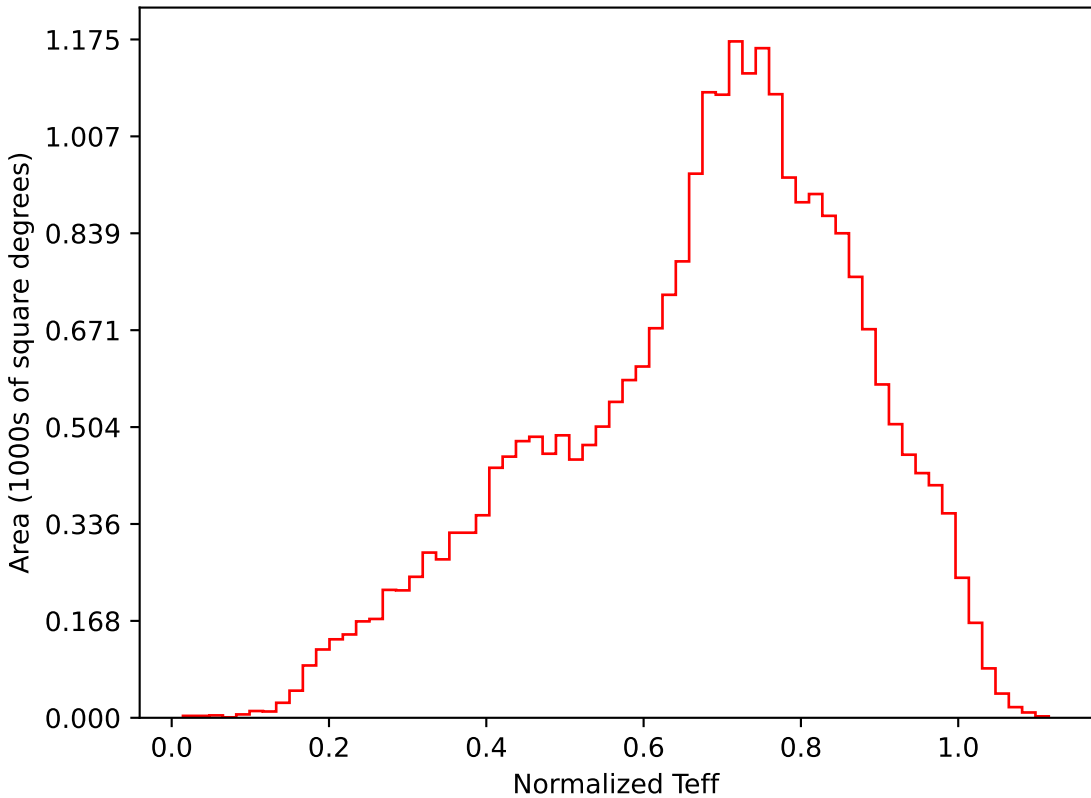
weather_cloudso2v3.4_10yrs All sky i band: Normalized Teff
