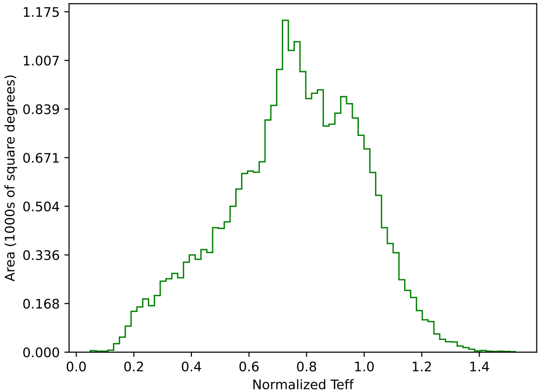
weather_cloudso2v3.4_10yrs All sky g band: Normalized Teff
