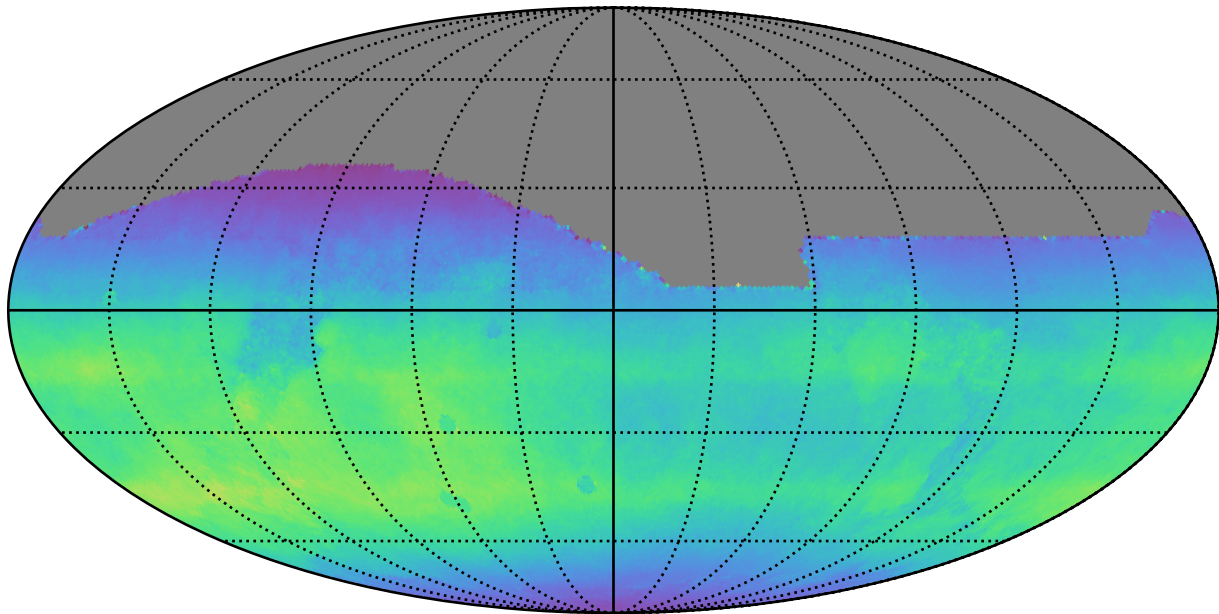
weather_cloudso2v3.4_10yrs All sky all bands: Normalized Teff
