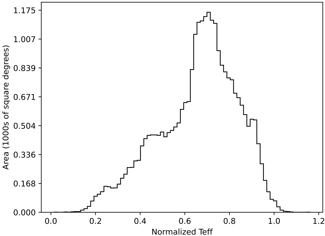
weather_cloudso2v3.4_10yrs All sky all bands: Normalized Teff
