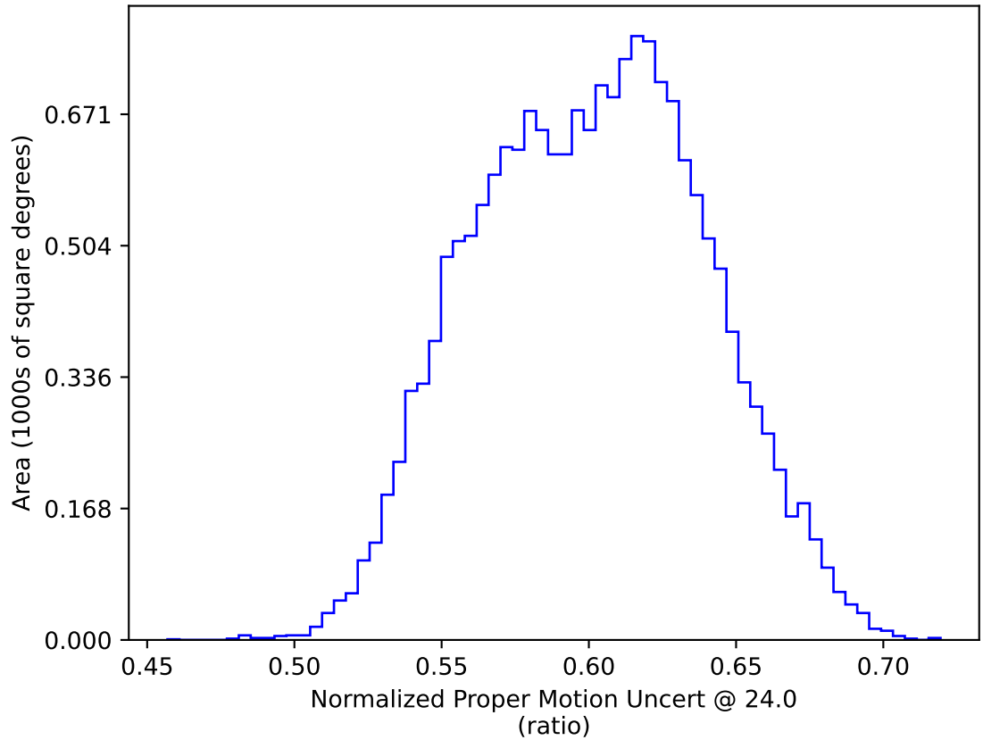
weather_cloudso2v3.4_10yrs WFD: Normalized Proper Motion Uncert @ 24.0
