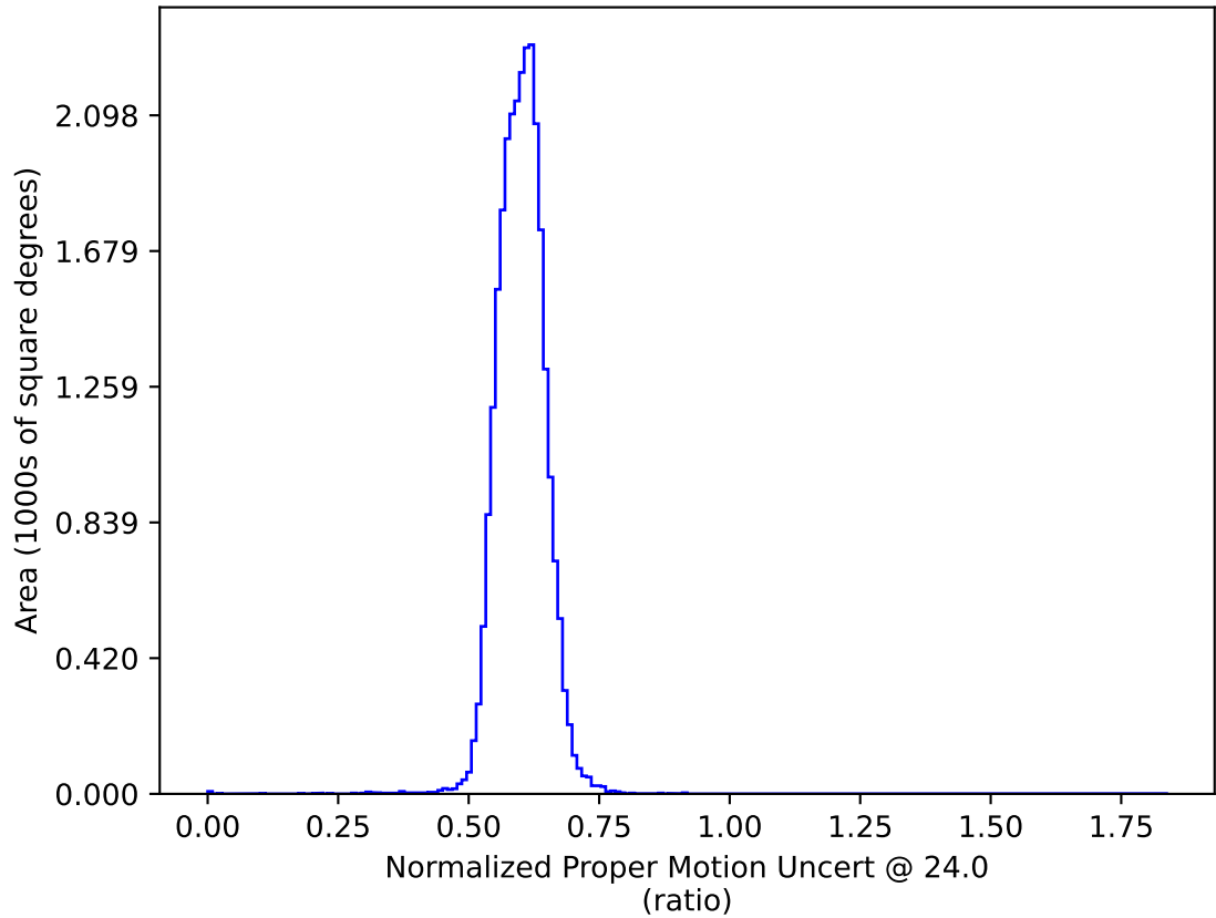
weather_cloudso2v3.4_10yrs All sky: Normalized Proper Motion Uncert @ 24.0
