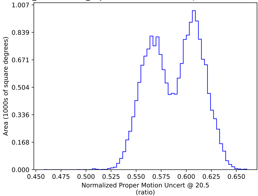
weather_cloudso2v3.4_10yrs WFD: Normalized Proper Motion Uncert @ 20.5
