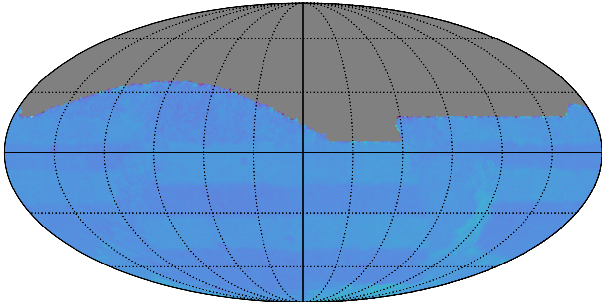
weather_cloudso2v3.4_10yrs All sky: Normalized Proper Motion Uncert @ 20.5
