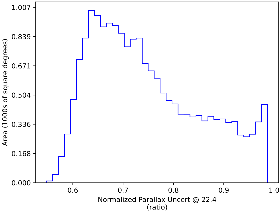
weather_cloudso2v3.4_10yrs WFD: Normalized Parallax Uncert @ 22.4
