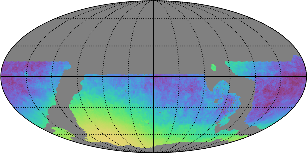
weather_cloudso2v3.4_10yrs WFD y band only: Normalized Parallax Uncert @ 21.3
