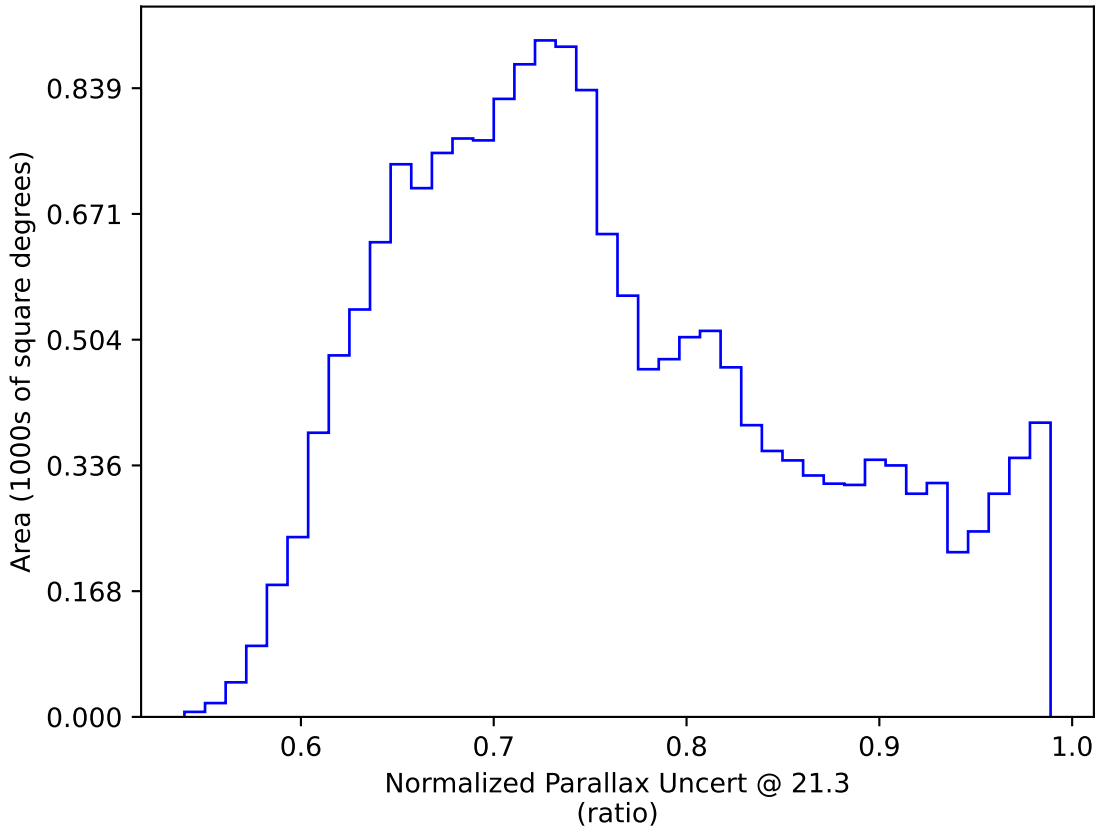
weather_cloudso2v3.4_10yrs WFD y band only: Normalized Parallax Uncert @ 21.3
