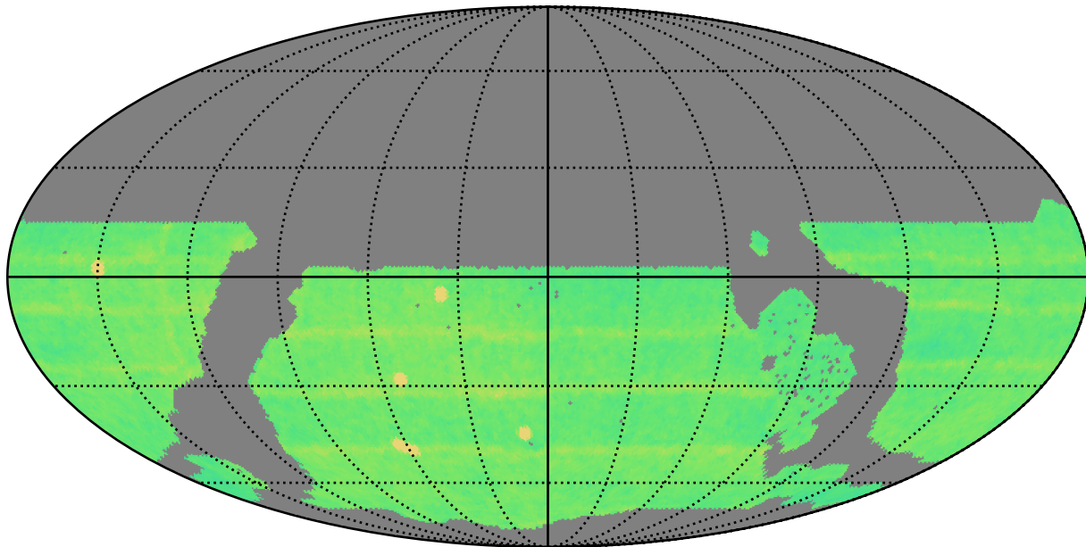
weather_cloudso2v3.4_10yrs WFD all bands: N Unique Nights
