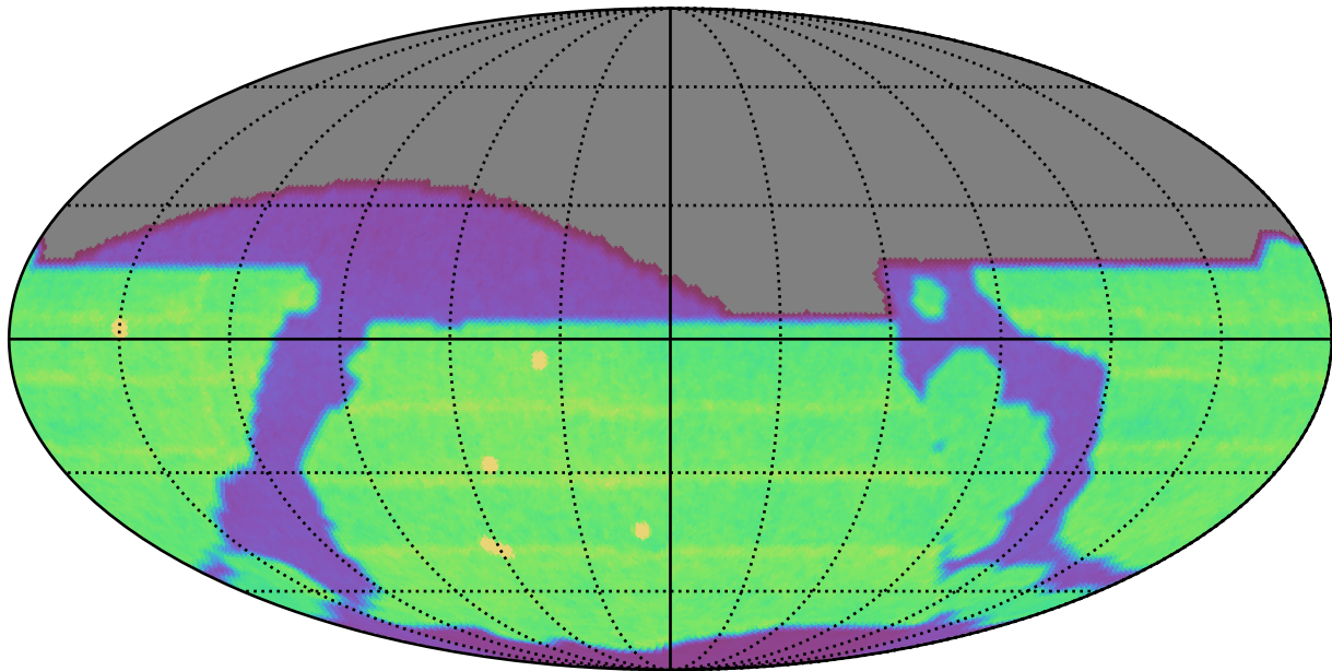
weather_cloudso2v3.4_10yrs All sky all bands: N Unique Nights
