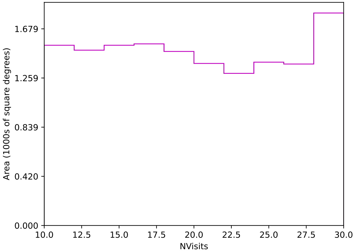
weather_cloudso2v3.4_10yrs Yr 3-4 z band: NVisits
