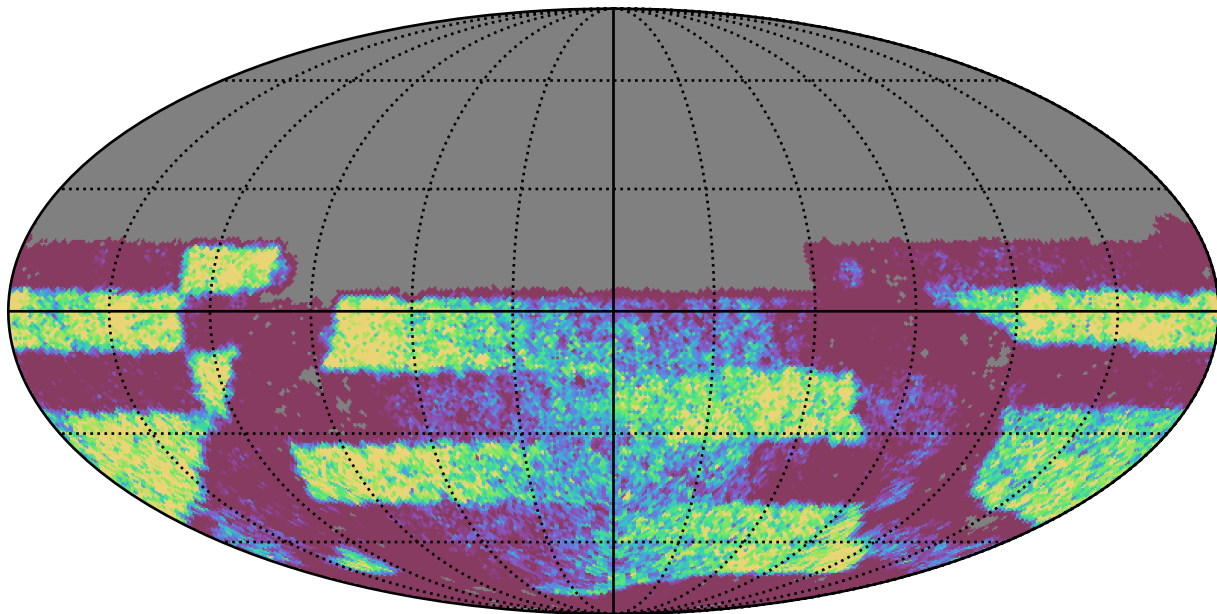
weather_cloudso2v3.4_10yrs Yr 3-4 y band: NVisits
