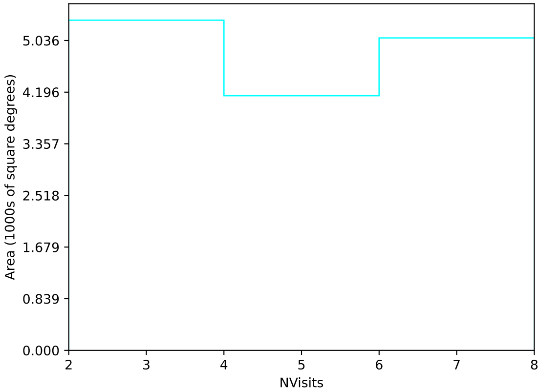
weather_cloudso2v3.4_10yrs Yr 3-4 u band: NVisits
