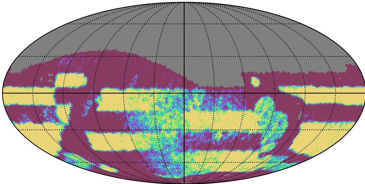
weather_cloudso2v3.4_10yrs Yr 3-4 r band: NVisits
