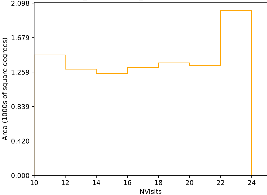
weather_cloudso2v3.4_10yrs Yr 3-4 r band: NVisits
