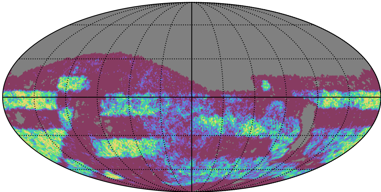
weather_cloudso2v3.4_10yrs Yr 3-4 g band: NVisits
