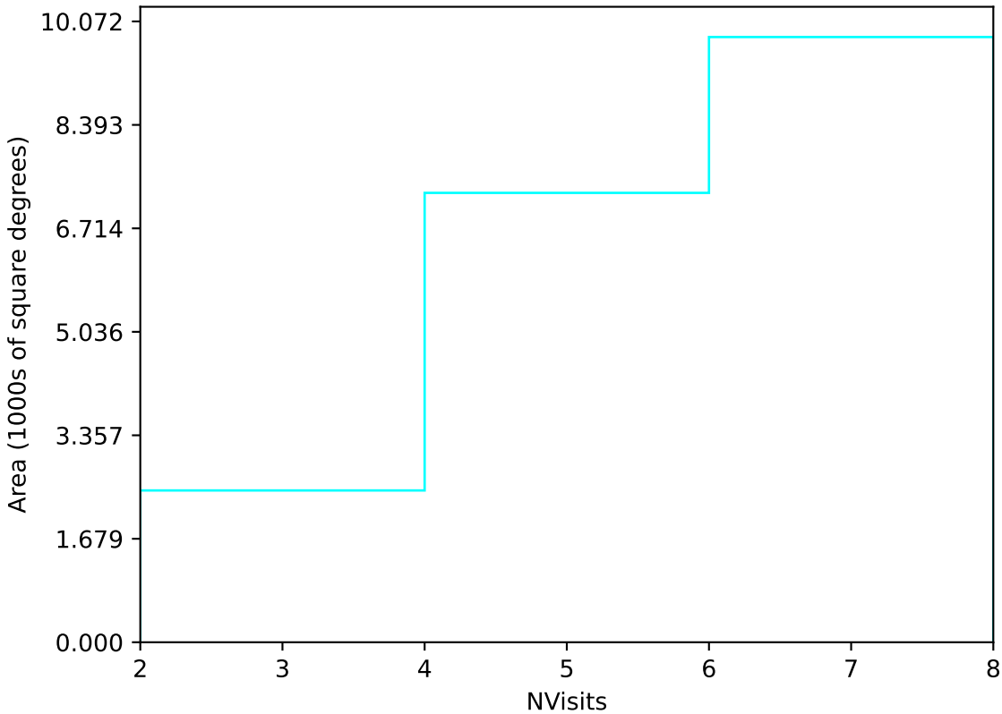
weather_cloudso2v3.4_10yrs Yr 1 u band: NVisits
