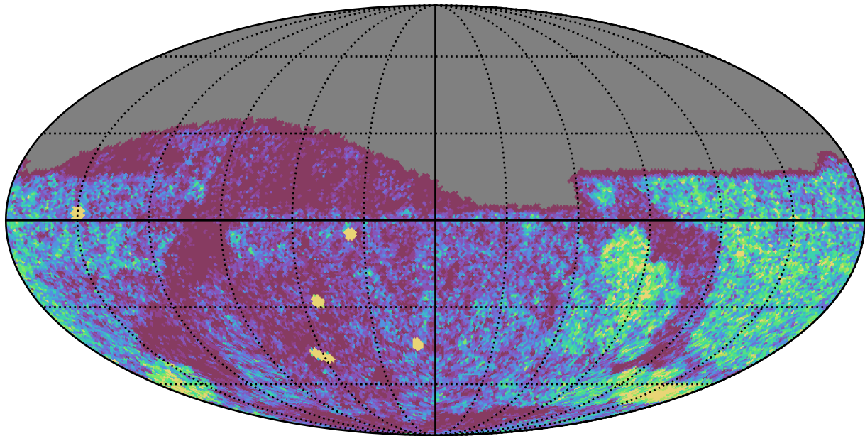
weather_cloudso2v3.4_10yrs Yr 1 g band: NVisits
