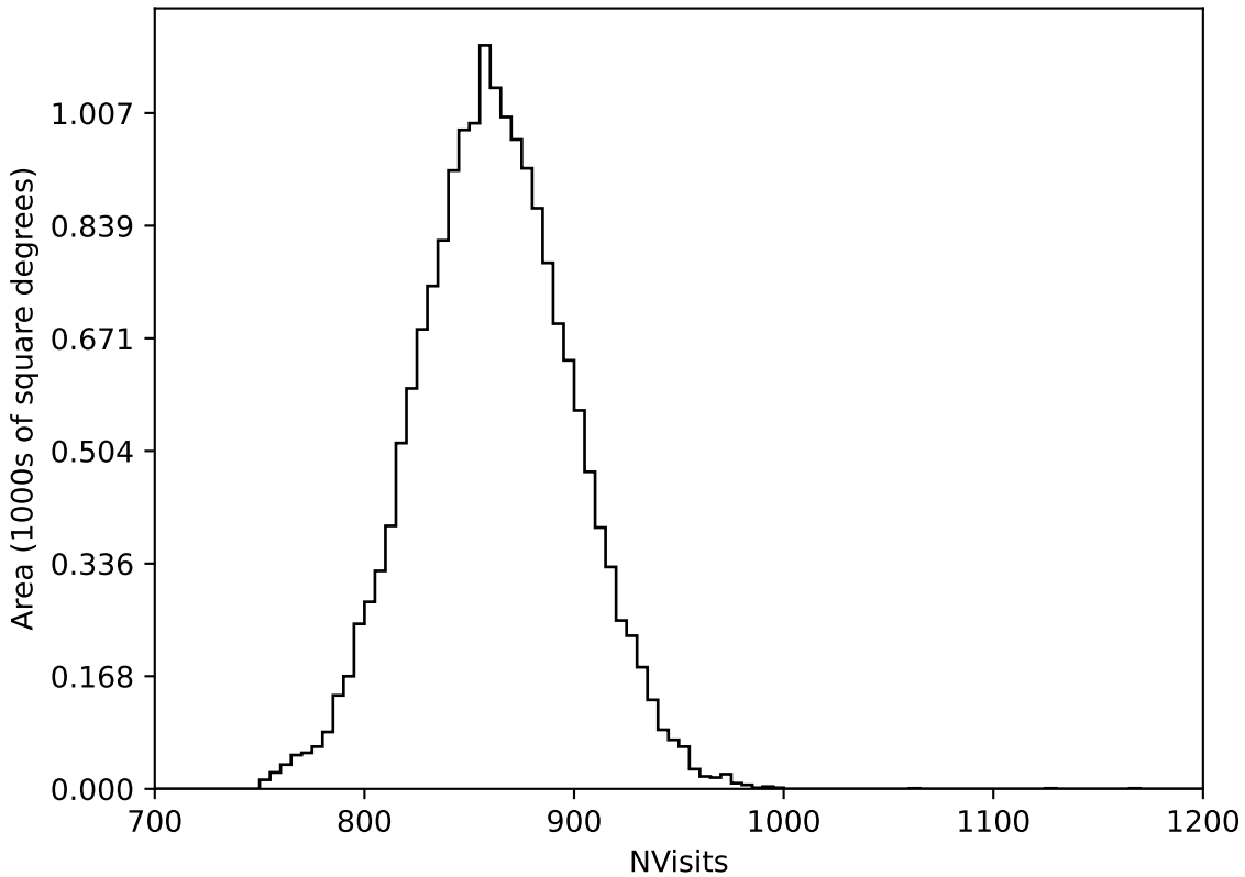
weather_cloudso2v3.4_10yrs WFD all bands: NVisits
