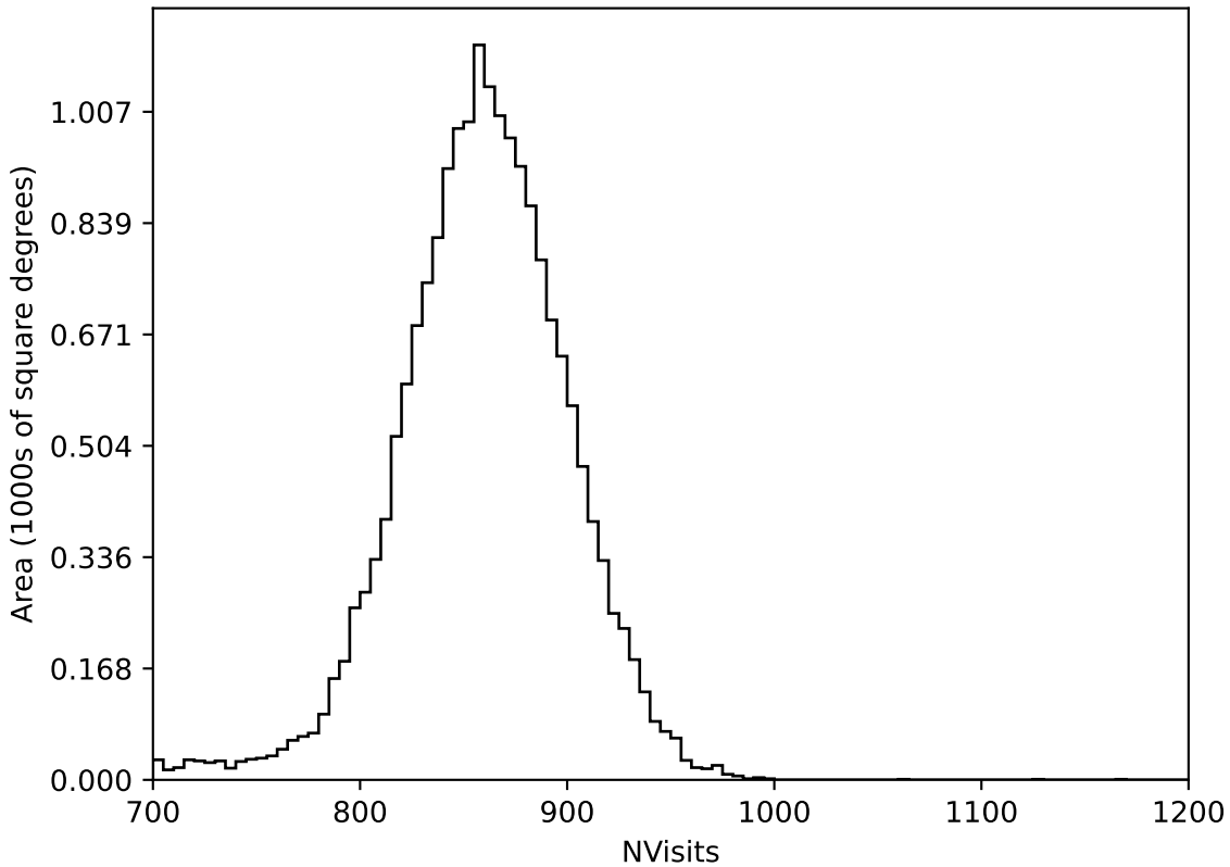
weather_cloudso2v3.4_10yrs All sky all bands: NVisits
