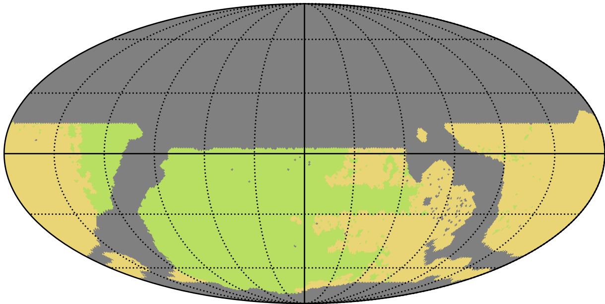
weather_cloudso2v3.4_10yrs WFD all bands: NSeasons
