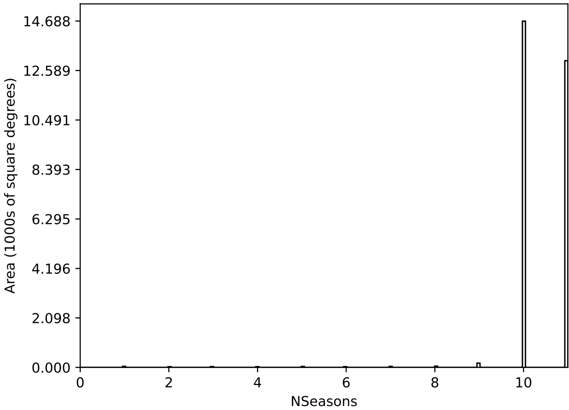
weather_cloudso2v3.4_10yrs All sky all bands: NSeasons
