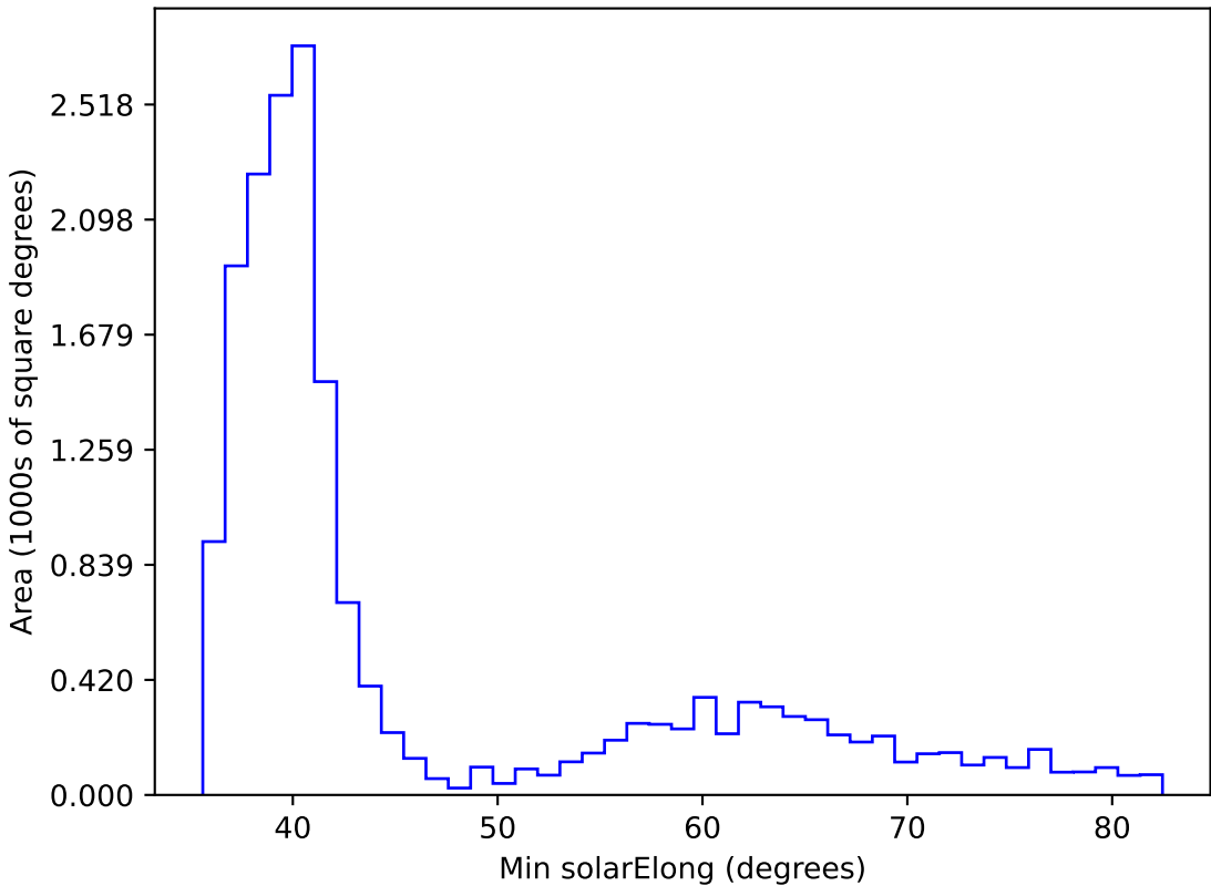
weather_cloudso2v3.4_10yrs WFD all bands: Min solarElong
