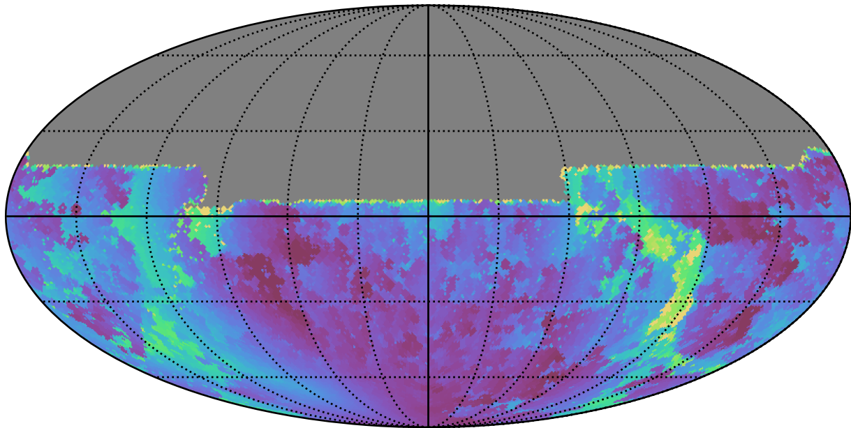
weather_cloudso2v3.4_10yrs All sky u band: Min solarElong
