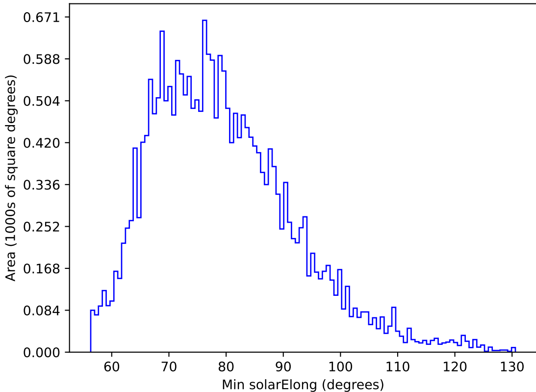
weather_cloudso2v3.4_10yrs All sky u band: Min solarElong
