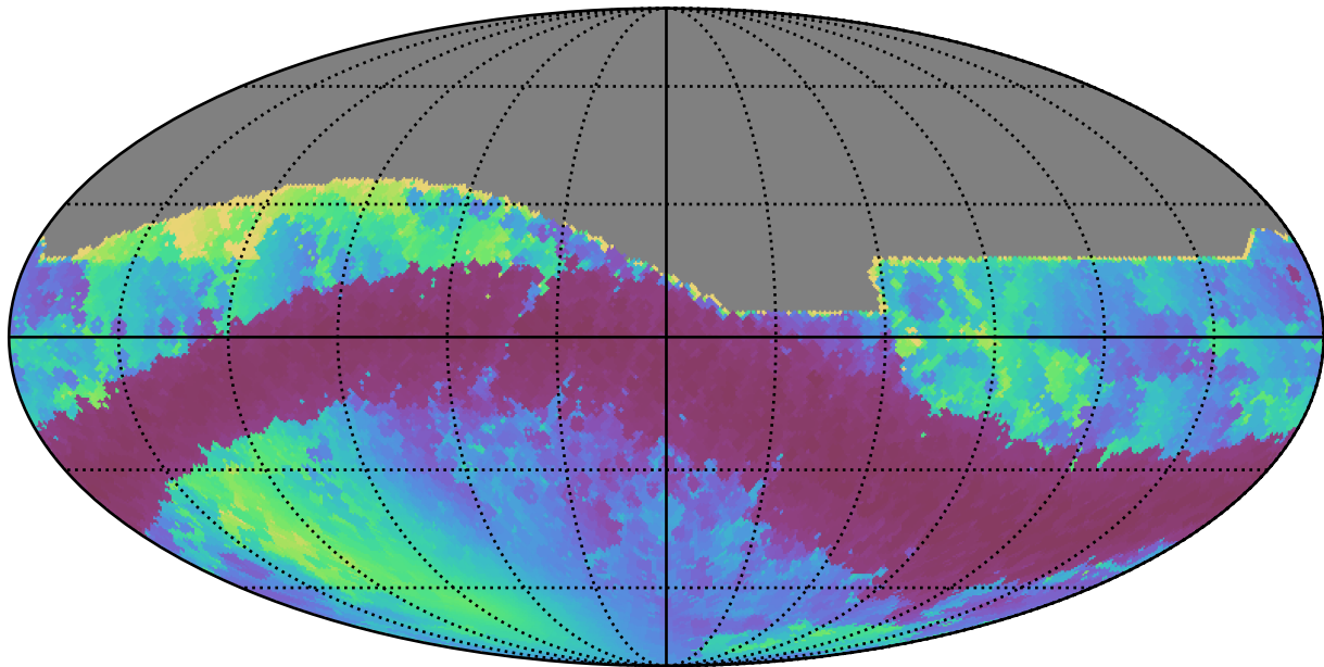
weather_cloudso2v3.4_10yrs All sky r band: Min solarElong
