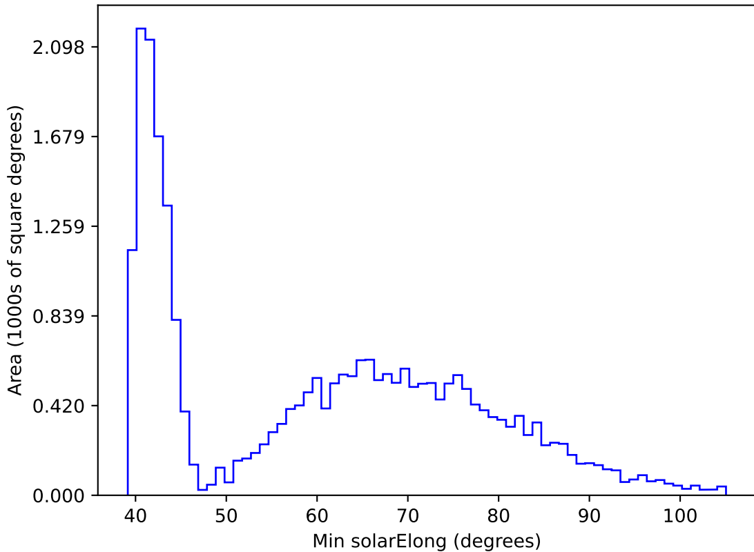
weather_cloudso2v3.4_10yrs All sky r band: Min solarElong
