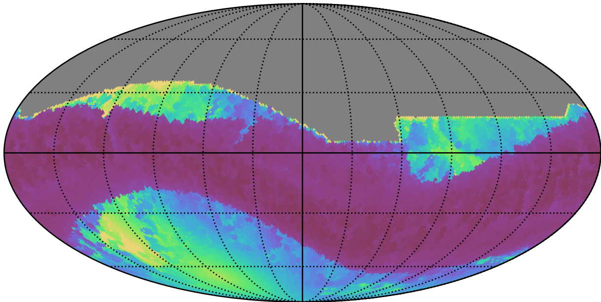
weather_cloudso2v3.4_10yrs All sky all bands: Min solarElong
