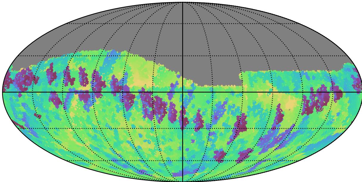
weather_cloudso2v3.4_10yrs Yr 1 z band: Min skyBrightness
