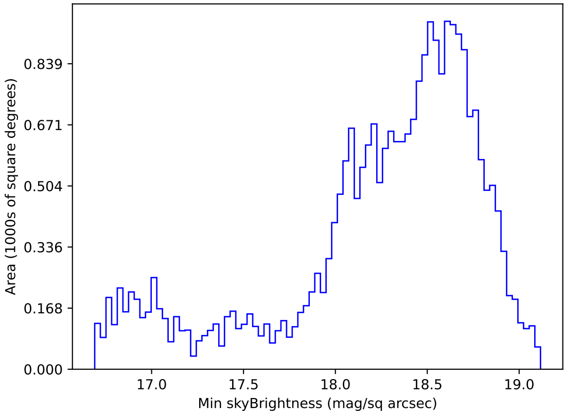
weather_cloudso2v3.4_10yrs Yr 1 z band: Min skyBrightness
